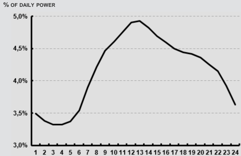
THE SHAPE OF THE GERMAN ELECTRIC LOAD IN AUGUST 2013 (SOURCE: ENTOSE)
