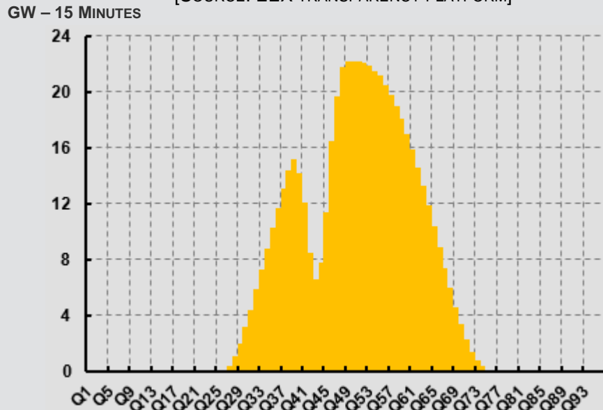
GERMAN SOLAR PV DAY-AHEAD FORECAST FOR DELIVERY FRIDAY MARCH 20, 2015 [SOURCE: EEX TRANSPARENCY PLATFORM]
