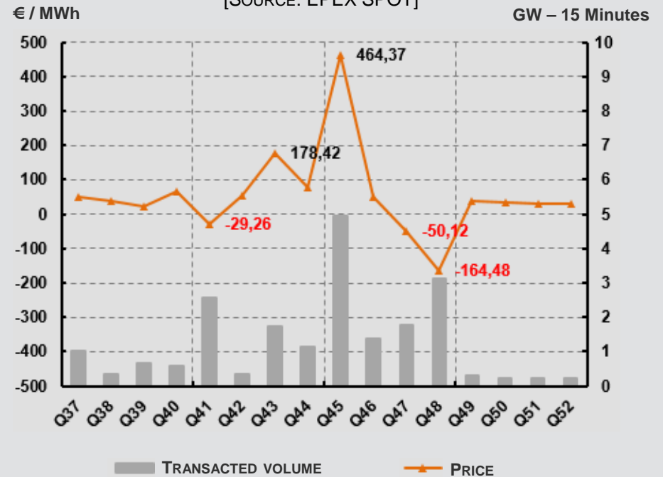
EPEX GERMANY 15 MINUTES AUCTION PRICES AND VOLUMES OVER THE ECLIPSE HOURS FRIDAY MARCH 20, 2015 [SOURCE: EPEX SPOT]
