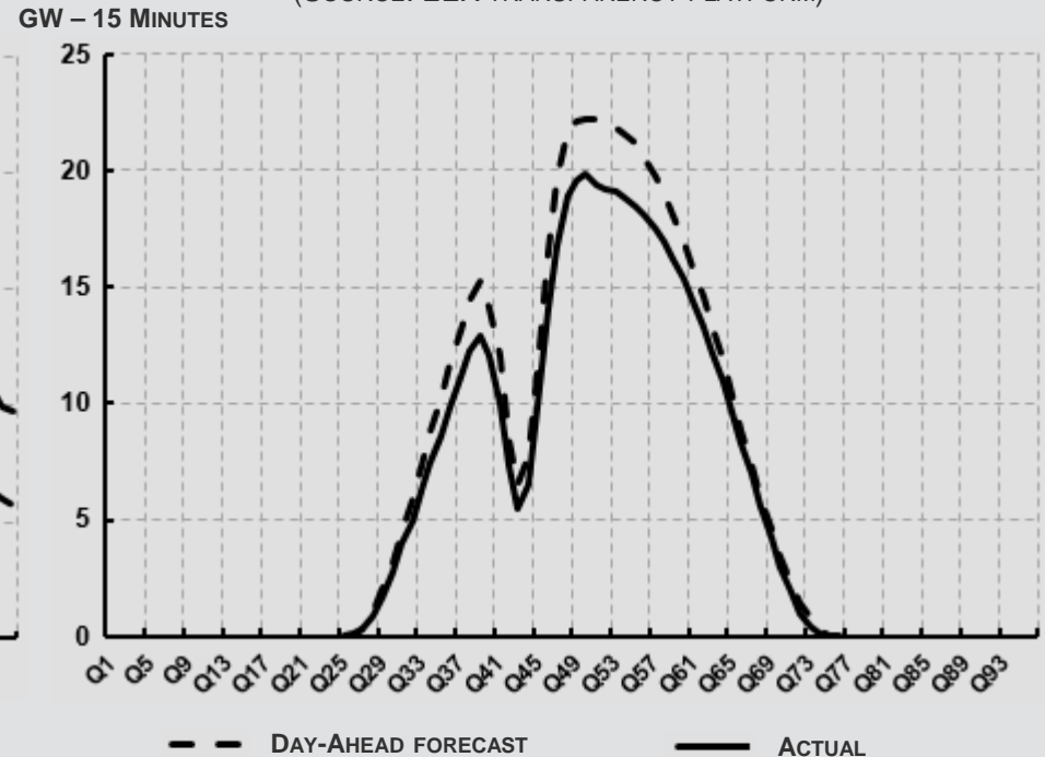
SOLAR PV DAY-AHEAD FORECAST VERSUS ACTUAL OUTPUT IN GERMANY ON MARCH 20, 2015 (SOURCE: EEX TRANSPARENCY PLATFORM)
