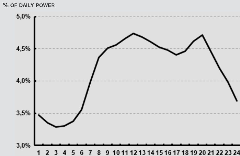
THE SHAPE OF THE GERMAN ELECTRIC LOAD IN OCTOBER 2013 (SOURCE: ENTOSE)
