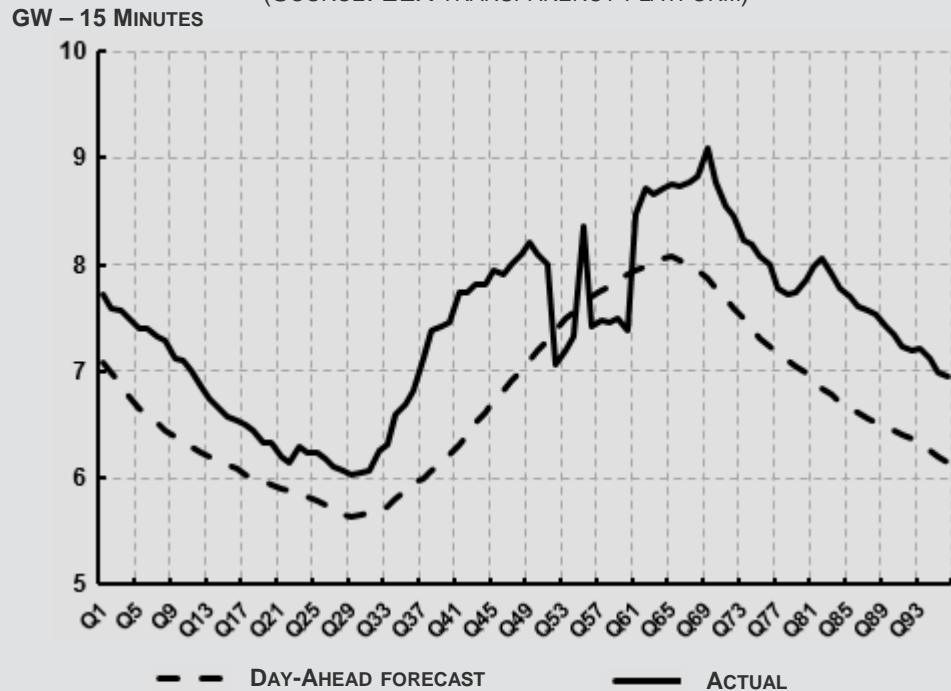
WIND ENERGY DAY-AHEAD FORECAST VERSUS ACTUAL OUTPUT IN TENNET CONTROL AREA ON MARCH 24, 2013 (SOURCE: EEX TRANSPARENCY PLATFORM)
